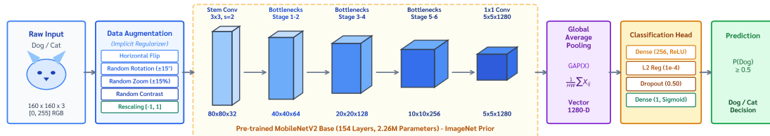
Panel (a): End-to-End Transfer Learning & Tensor Dataflow Pipeline (MobileNetV2 Backbone)
