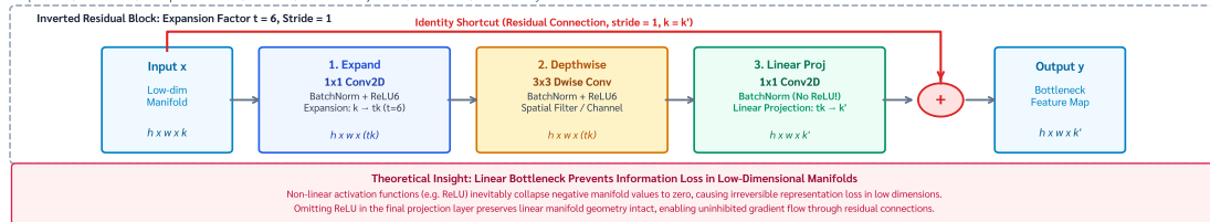
Panel (b): MobileNetV2 Inverted Residual Block with Linear Bottleneck (Micro-Architecture)
